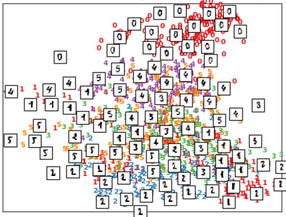
Random forest embedding of the digits (time 0.19s)
