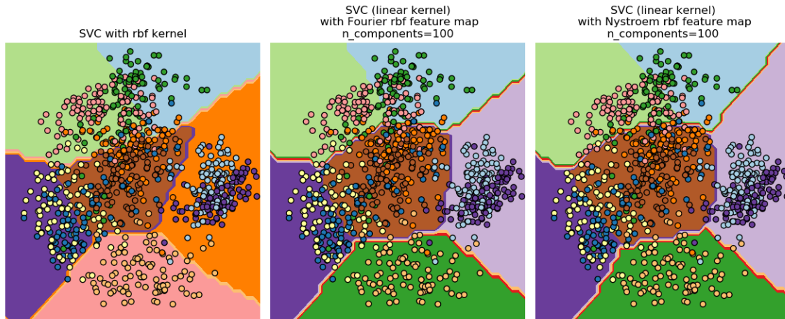
Fig. 3.9: Comparing an exact RBF kernel (left) with the approximation (right)
