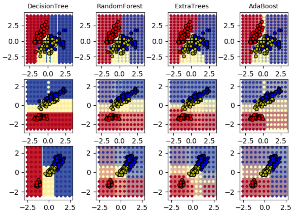
Classifiers on feature subsets of the Iris dataset
