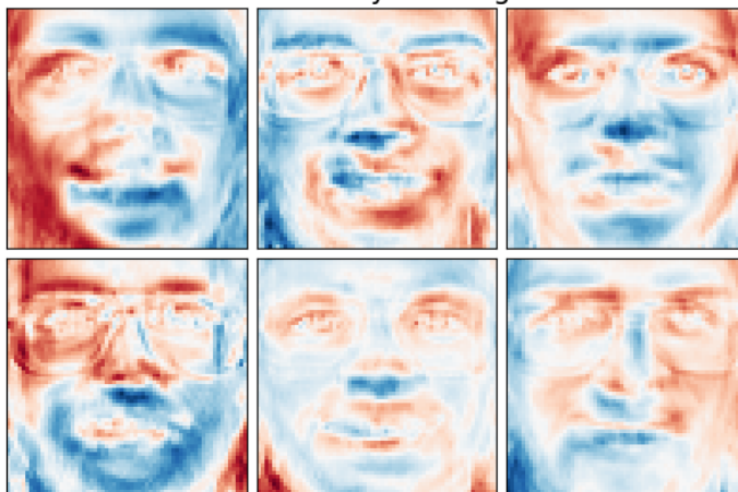
Dictionary learning
