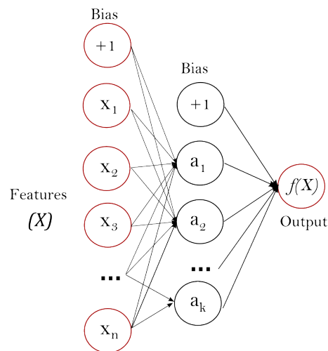
Fig. 3.2: Figure 1 : One hidden layer MLP.
