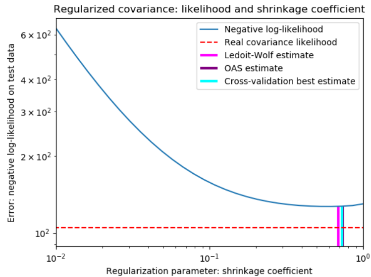
Fig. 3.7: Bias-variance trade-off when setting the shrinkage: comparing the choices of Ledoit-Wolf and OAS estimators
