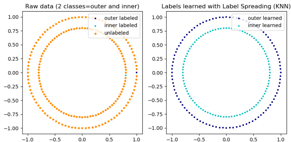
Fig. 3.1: An illustration of label-propagation: the structure of unlabeled observations is consistent with the class structure, and thus the class label can be propagated to the unlabeled observations of the training set.
