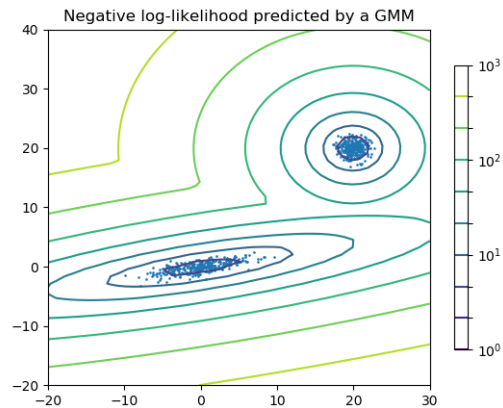
Fig. 3.3: Two-component Gaussian mixture model: data points, and equi-probability surfaces of the model.
